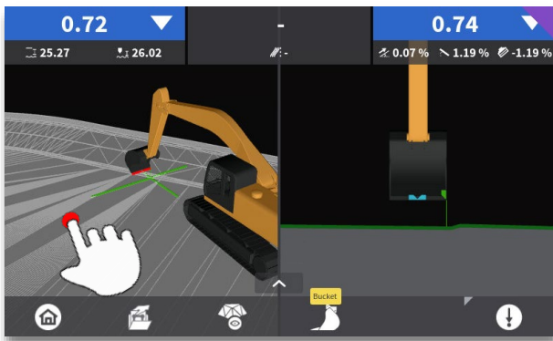
Step 1: Press and hold on plan view to see the "References" menu.
